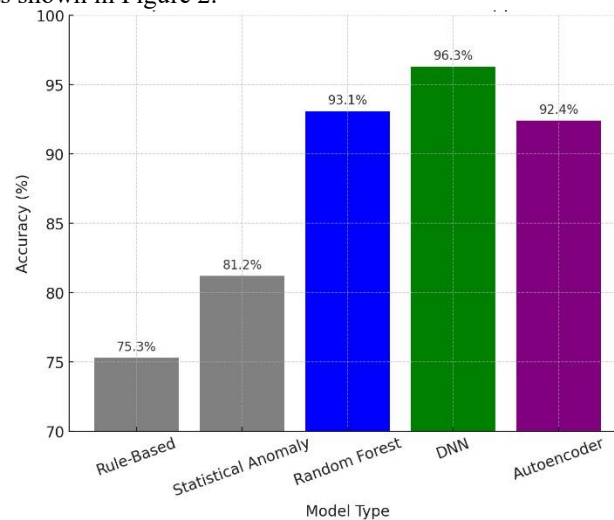
Figure 2: Performance Comparison with Baseline Systems
