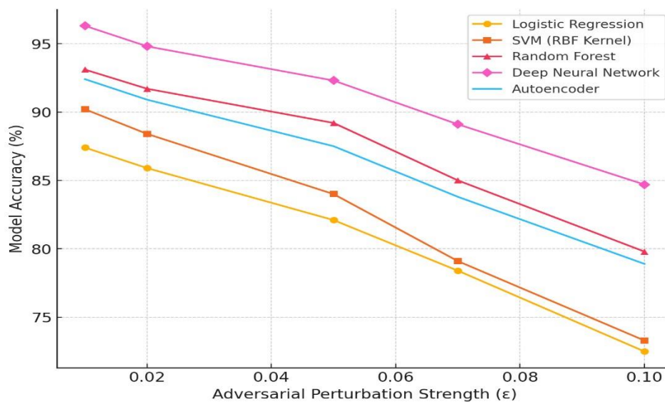
Figure 1: Adversarial Attack Impact on Model Accuracy
